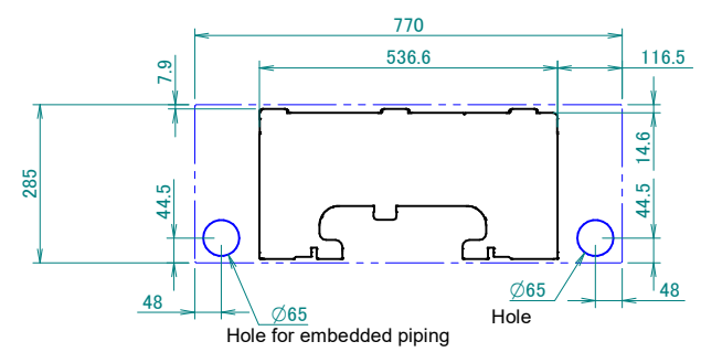
Standard location of holes in the wall
